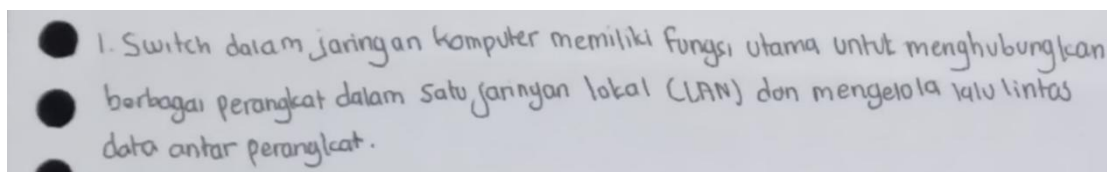
Figure 4 Using AI
